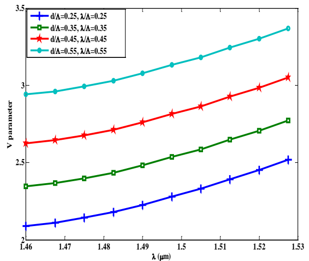
Fig. 2: (a). V parameter vs. wavelength for different values of d/\Lambda and \lambda/\Lambda at S communication band (silicon)
